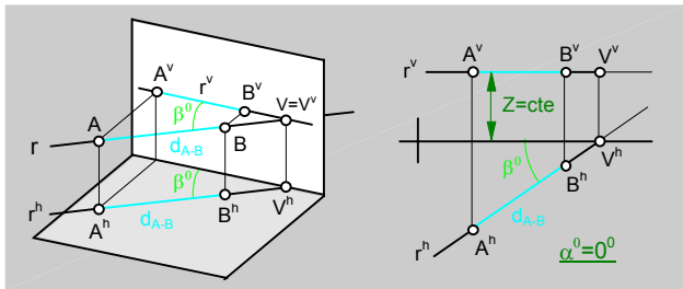
fig.94.\ Recta horizontal.
