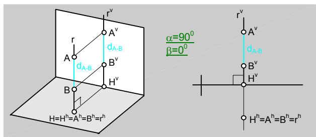
fig.100.\ Recta vertical.
