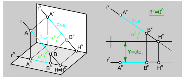
fig.96.\ Recta frontal.
